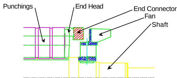
FIG. 3 - CuBar Rotor Cutaway View
