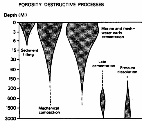
Figure 18.8 Schematic illustration of the relationship between depth and the major porosity-forming and porosity-destroying processes. After Longman (1982)
