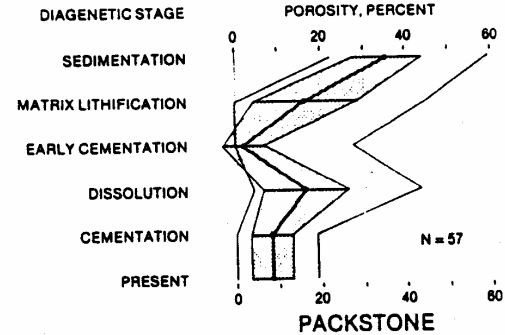
Fig. 22. Porosity evolution of packstone in Poza Rica trend. Conventions as in Fig. 21.
