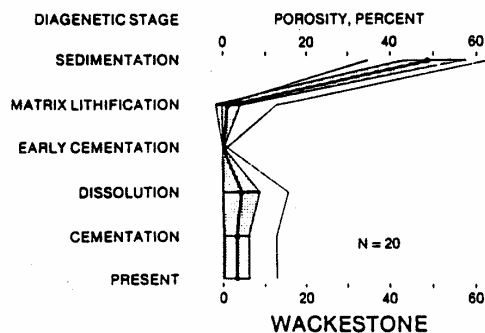
Fig. 23. Porosity evolution of wackestone in Poza Rica trend. Conventions as in Fig. 21.
