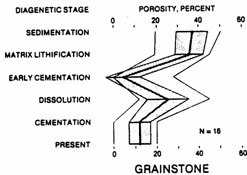
Fig. 21. Summary of porosity evolution in grainstone of the Poza Rica trend. The abscissa indicates the porosity at the close of each diagenetic stage, listed sequentially in the ordinate beginning at the top. Bold line shows the arithmetic mean value at the close of each diagenetic stage. The shaded area includes one standard deviation about the mean. The outside envelope shows the maximum and minimum values at each stage; this is not the path of a single sample, but the extremes at each stage.
