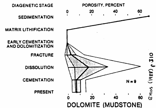
Fig. 24. Porosity evolution of dolomite in Poza Rica trend. The depositional texture is presumed to have been mudstone based on the small portion of recognizable grains. The high portion of mud and the assumption that mud had 70% porosity produces the artificially narrow range of variation through the first two diagenetic stages. Conventions are as in Fig. 21.
